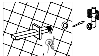
Wrap the thread of spout with teflon tape (ensure it must warp clockwise). Screw-in to the inlet pipe inside the wall, then install the decorative cover on the wall clingy.
